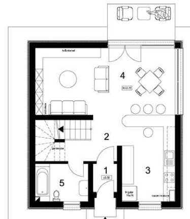
Plan parter TIP B, casa 1,2,3,4,5,10, 11,12,13,17 - scara 1/200
