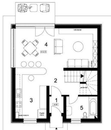
Plan parter TIP A, casa 6,7,8,9,14, 15,16,18,19,20 - scara 1/200
